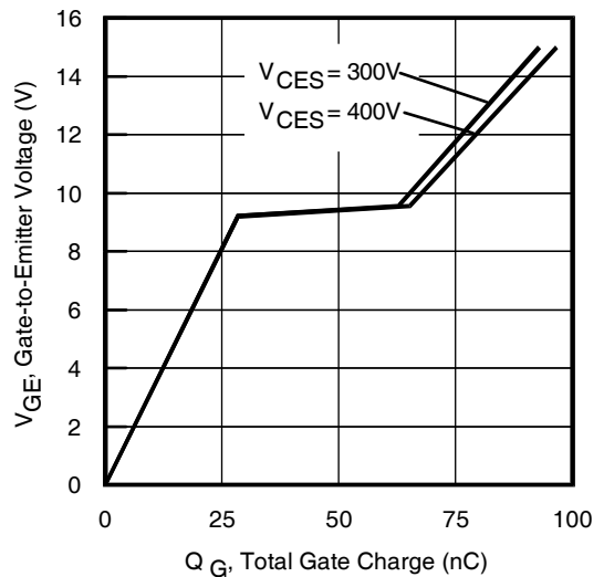
Fig. 24 - Typical Gate Charge vs. V_{GE} I_C = 48A ; L = 600uH
